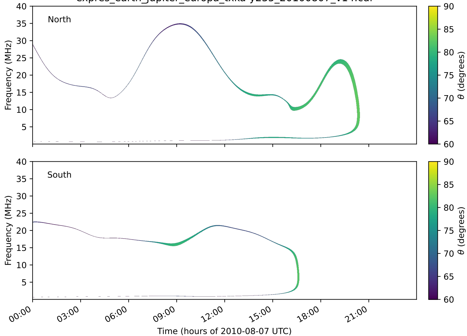
expres_earth_jupiter_europa_txka-y235_20100807_v14.cdf
