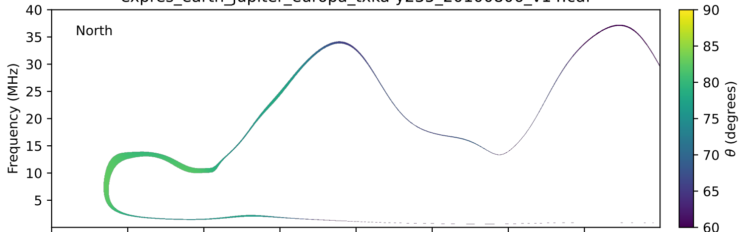
expres_earth_jupiter_europa_txka-y235_20100806_v14.cdf
