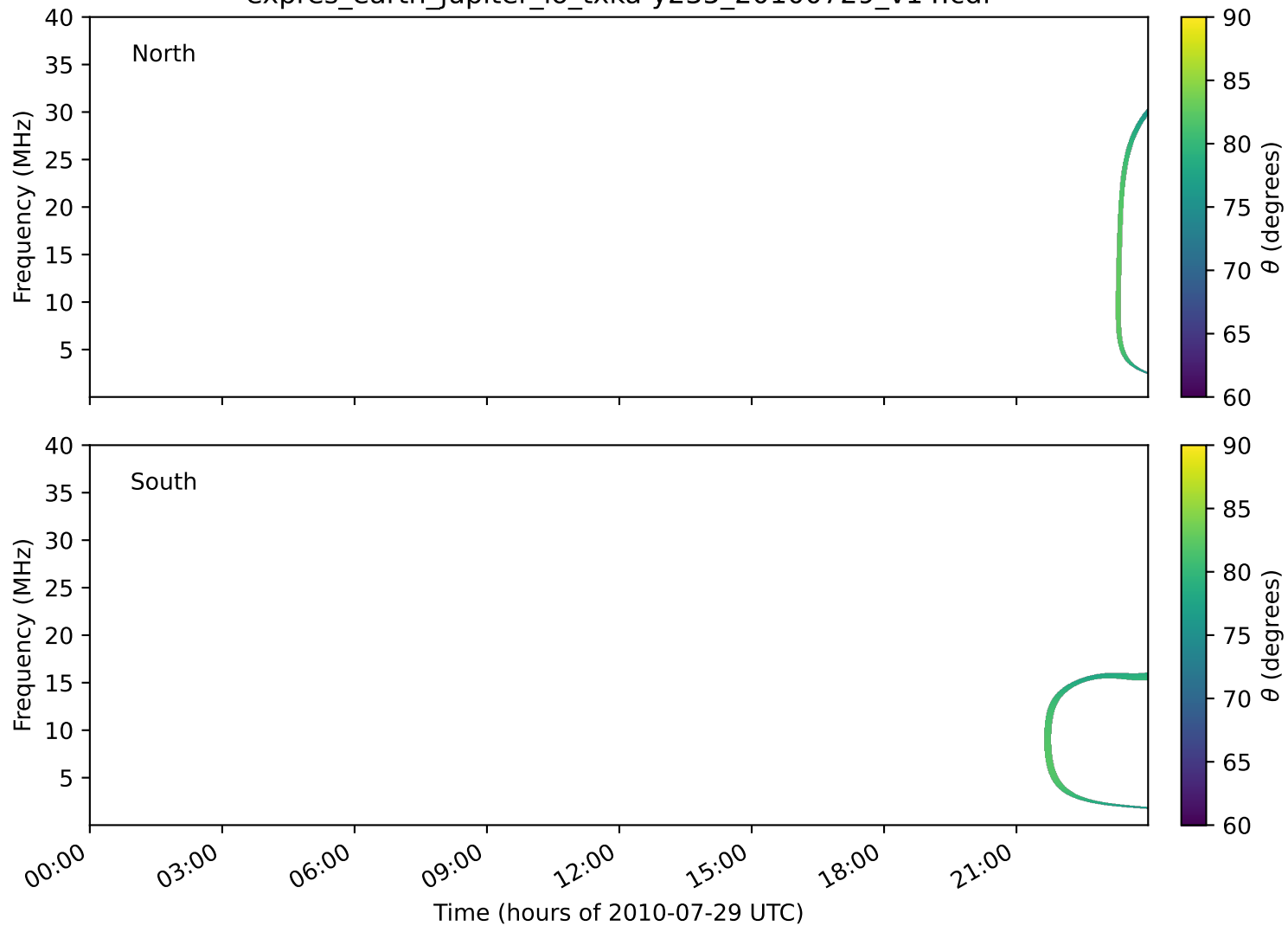
expres_earth_jupiter_io_txka-y235_20100729_v14.cdf
