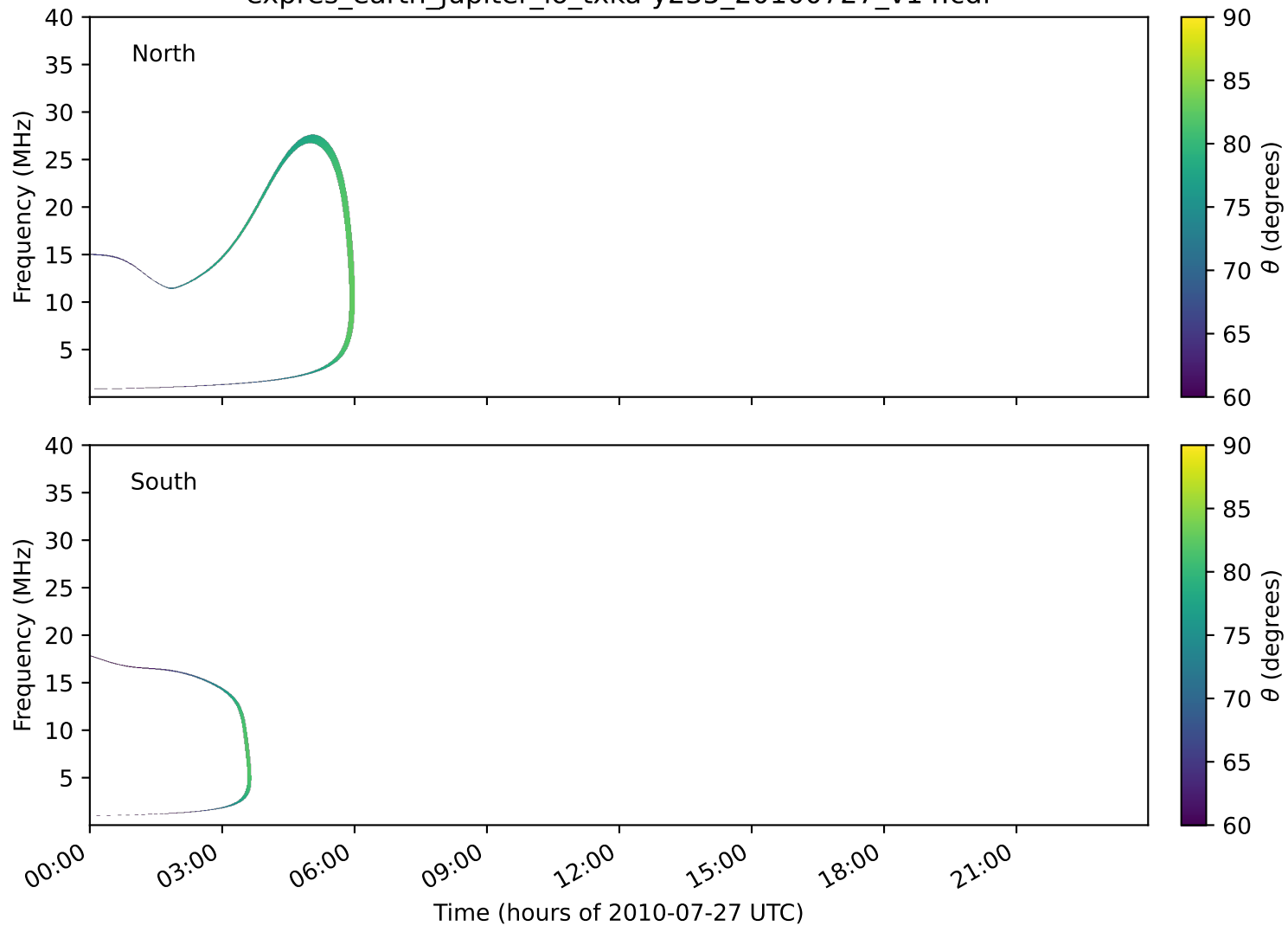
expres_earth_jupiter_io_txka-y235_20100727_v14.cdf
