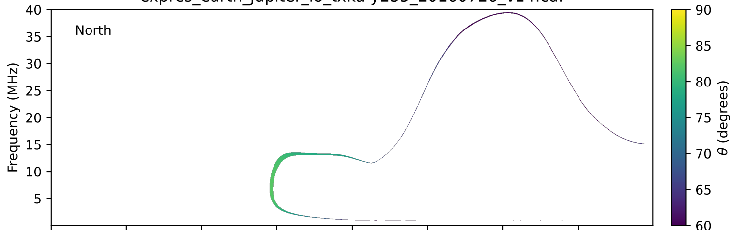
expres_earth_jupiter_io_txka-y235_20100726_v14.cdf
