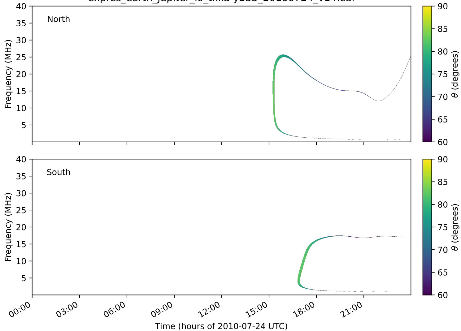
expres_earth_jupiter_io_txka-y235_20100724_v14.cdf
