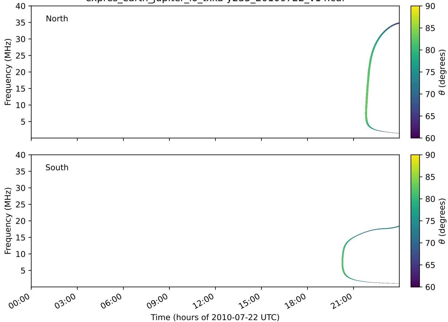
expres_earth_jupiter_io_txka-y235_20100722_v14.cdf
