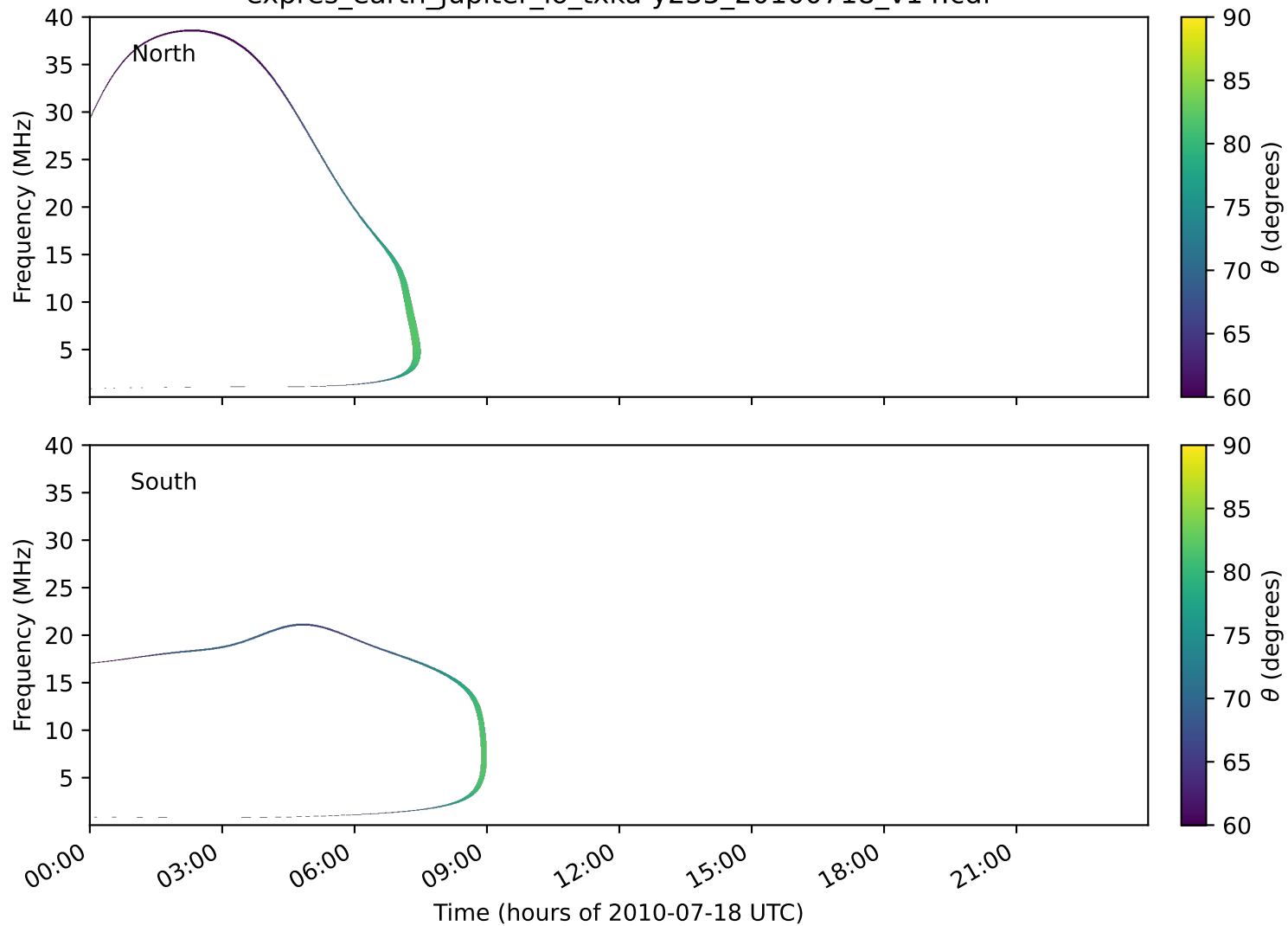
expres_earth_jupiter_io_txka-y235_20100718_v14.cdf
