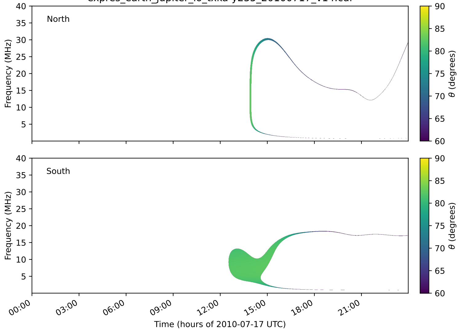
expres_earth_jupiter_io_txka-y235_20100717_v14.cdf
