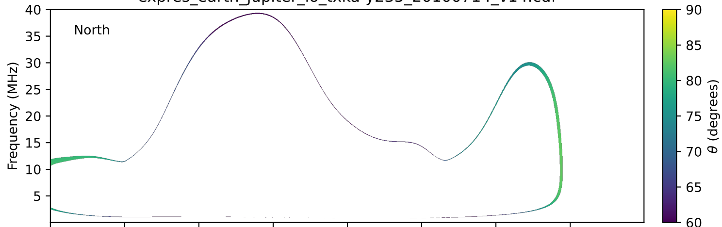
expres_earth_jupiter_io_txka-y235_20100714_v14.cdf
