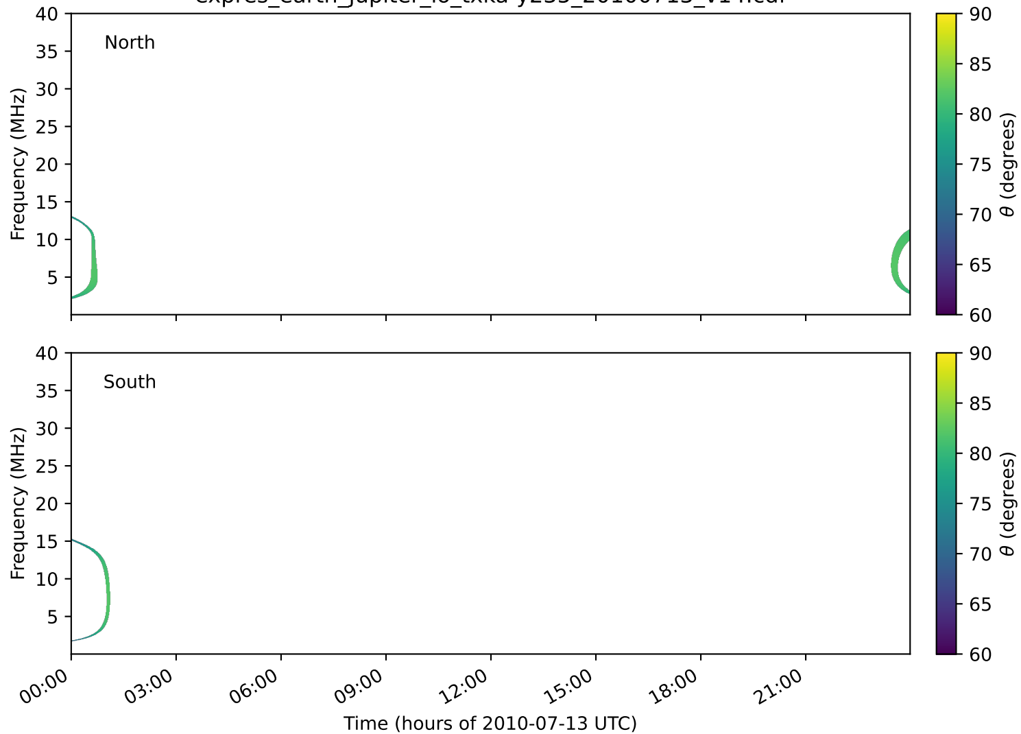
expres_earth_jupiter_io_txka-y235_20100713_v14.cdf
