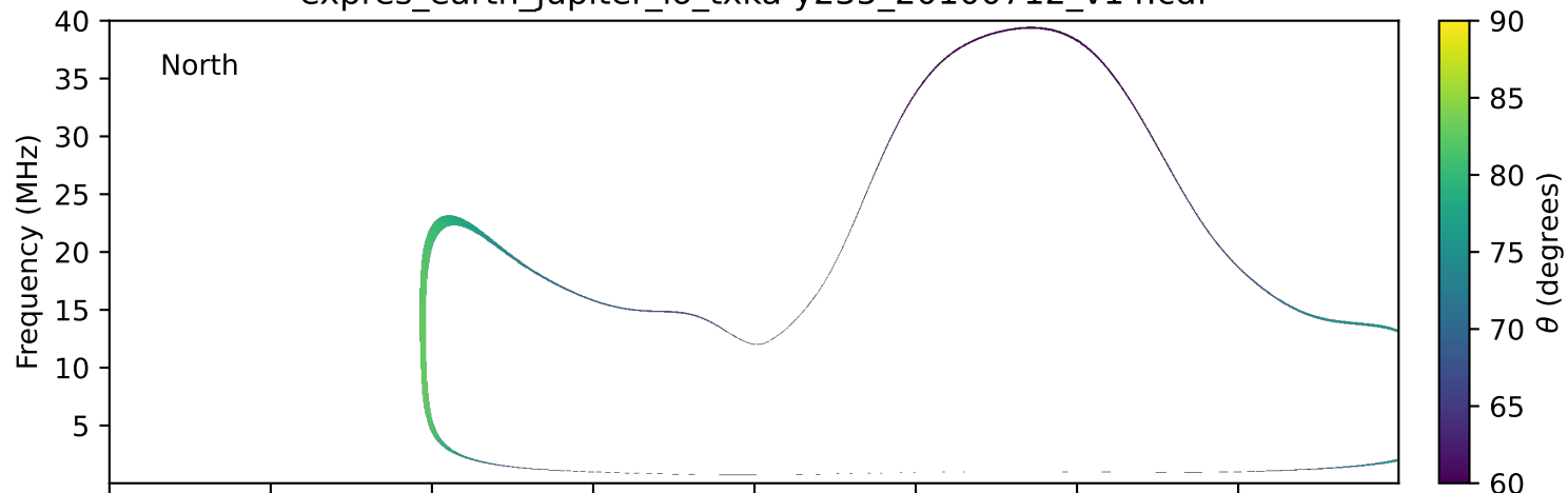
expres_earth_jupiter_io_txka-y235_20100712_v14.cdf
