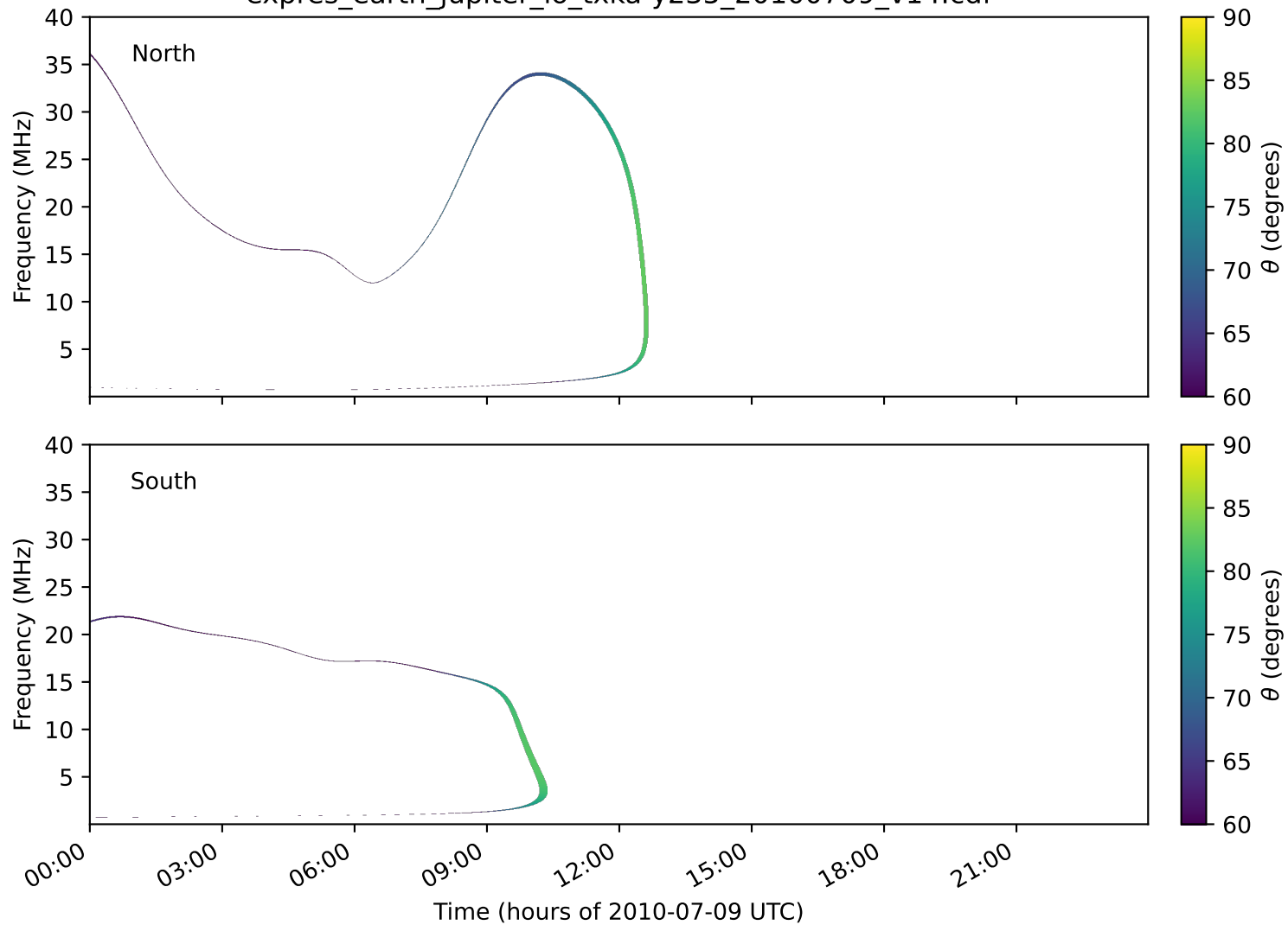
expres_earth_jupiter_io_txka-y235_20100709_v14.cdf
