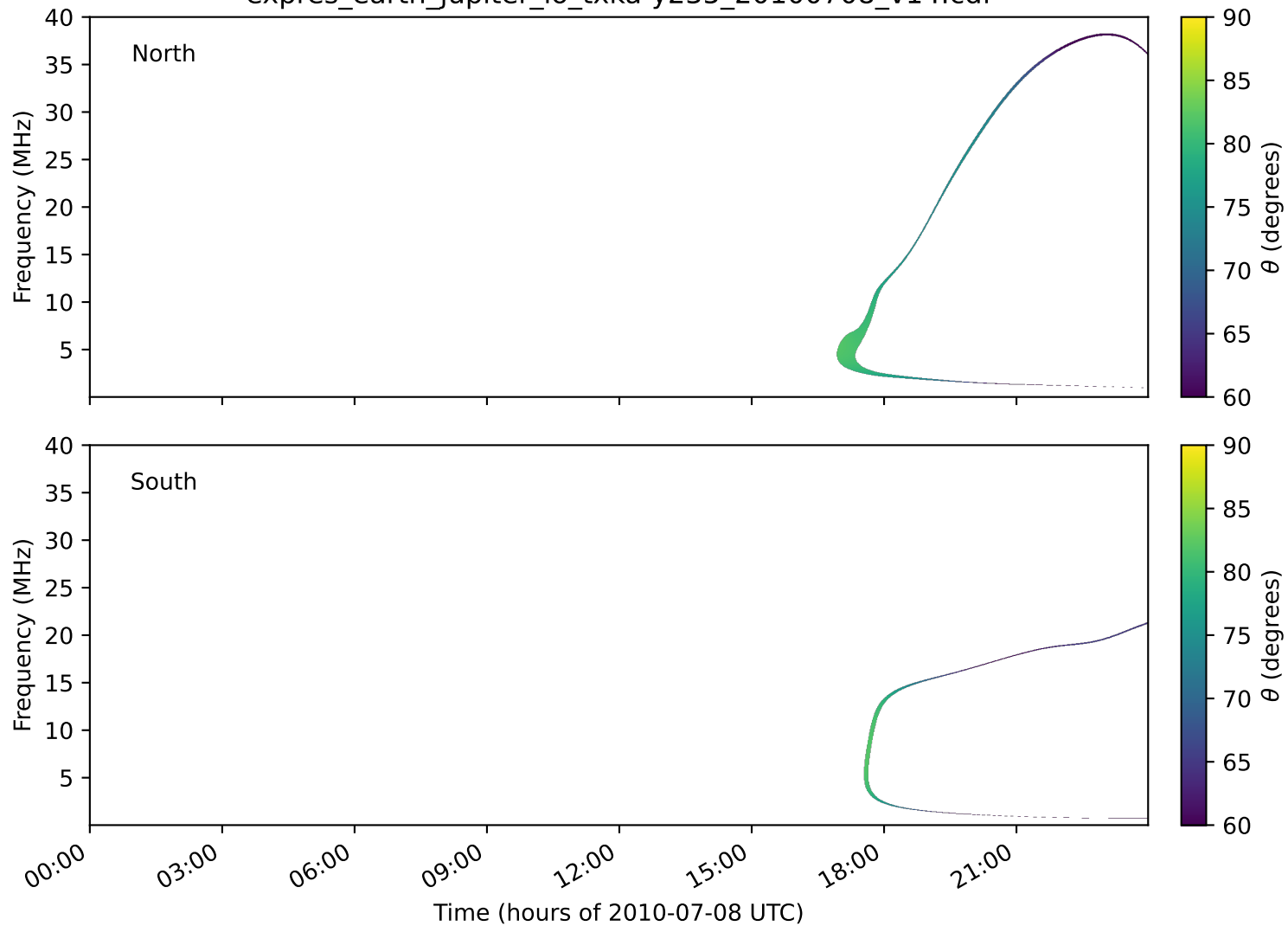
expres_earth_jupiter_io_txka-y235_20100708_v14.cdf
