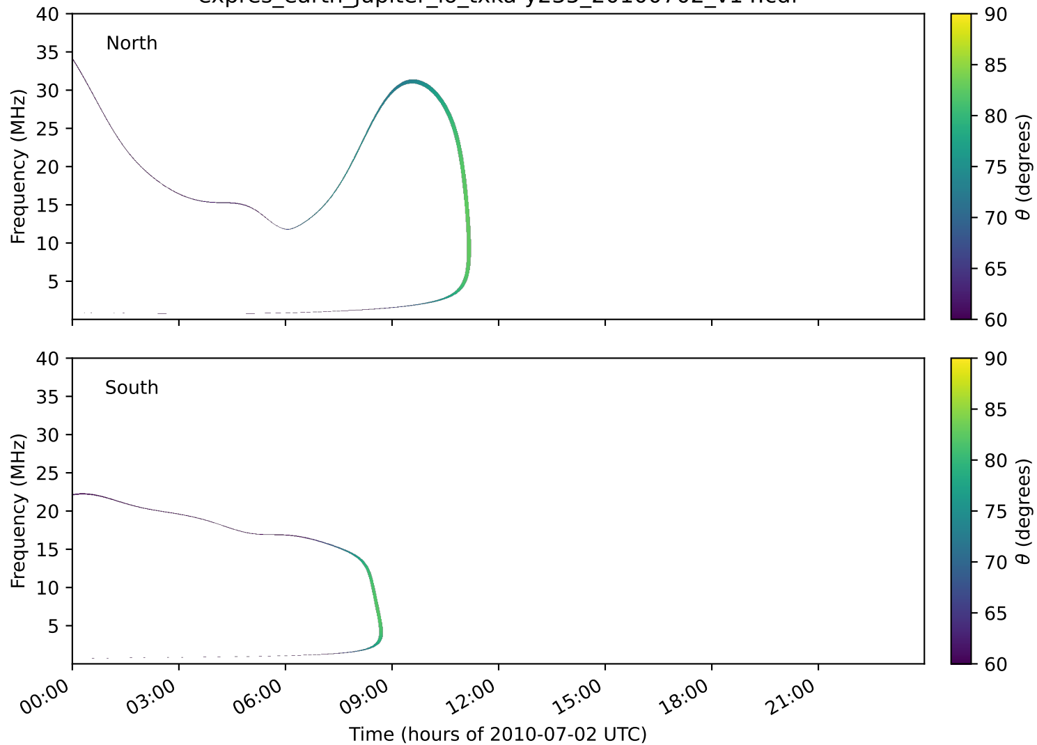
expres_earth_jupiter_io_txka-y235_20100702_v14.cdf
