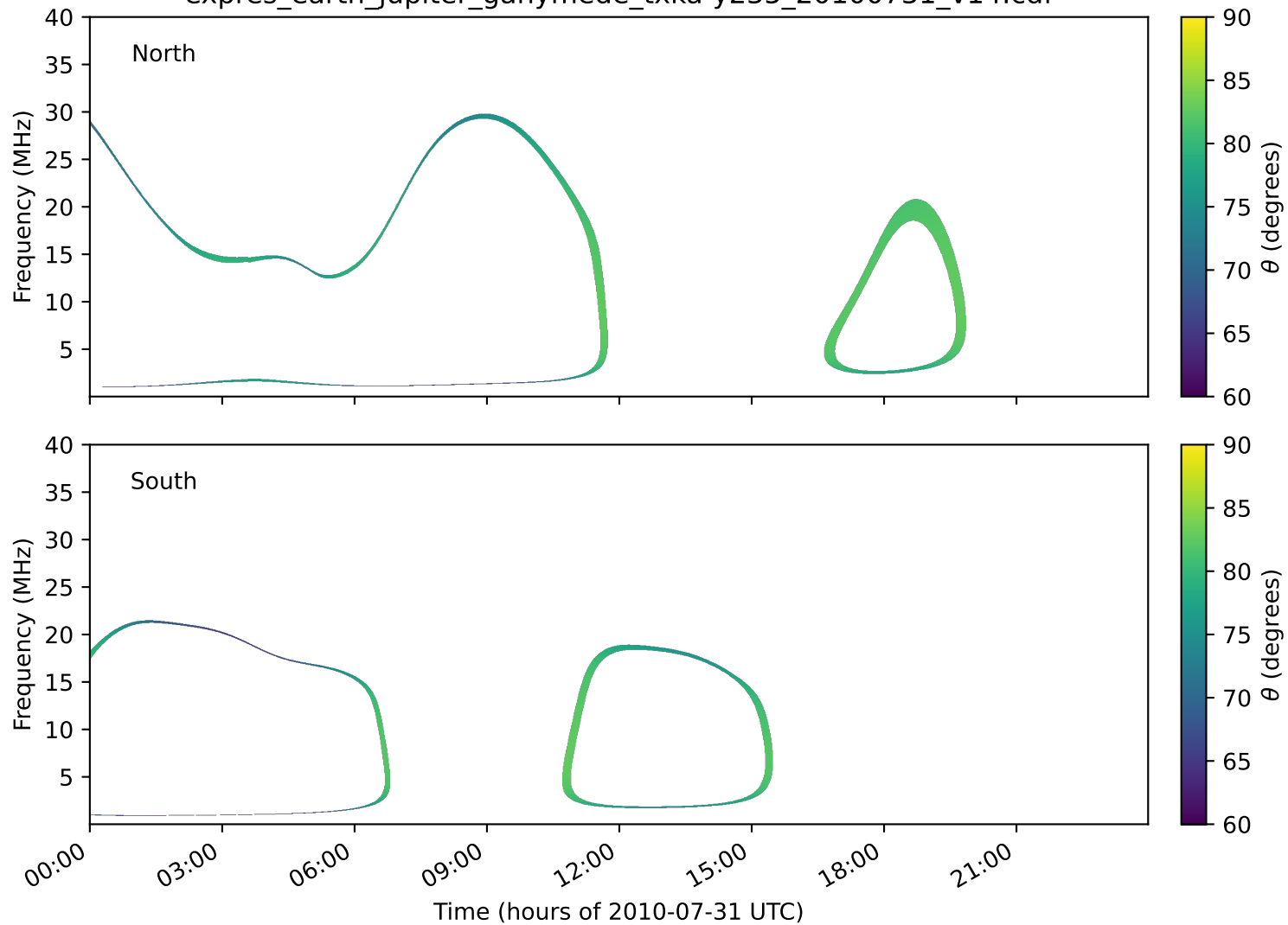
expres_earth_jupiter_ganymede_txka-y235_20100731_v14.cdf
