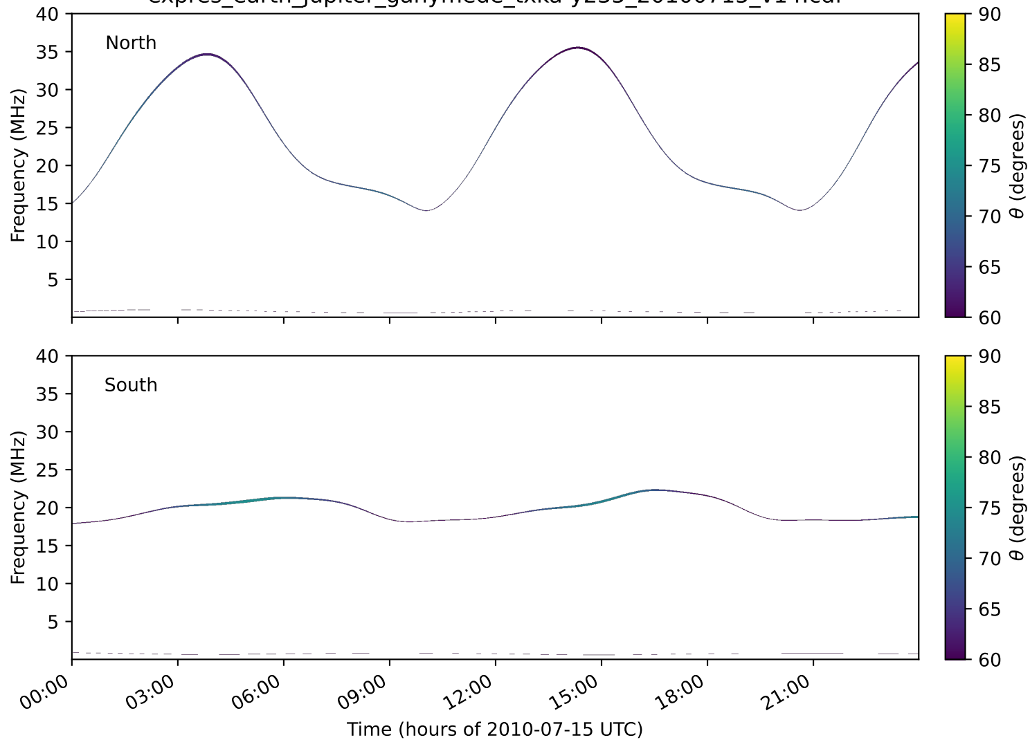
expres_earth_jupiter_ganymede_txka-y235_20100715_v14.cdf
