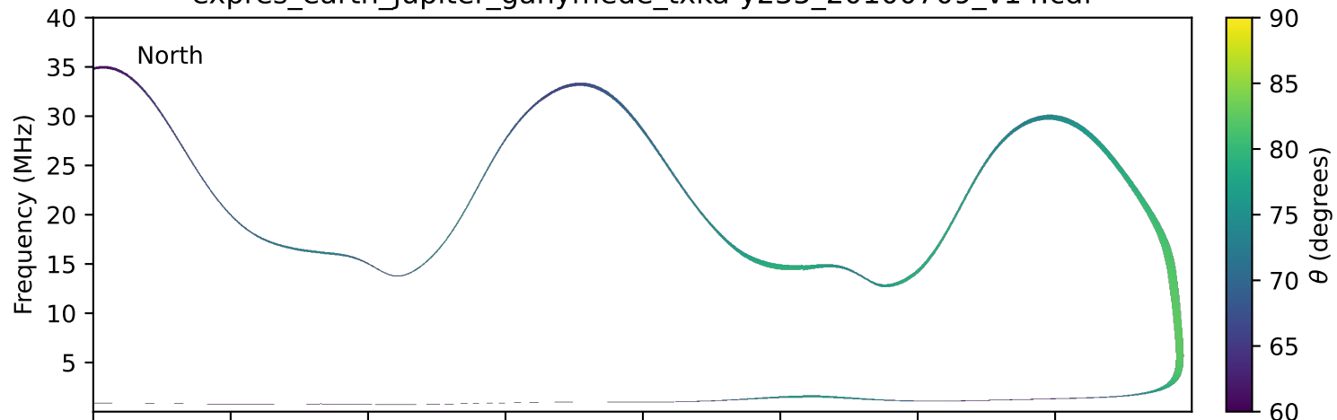
expres_earth_jupiter_ganymede_txka-y235_20100709_v14.cdf
