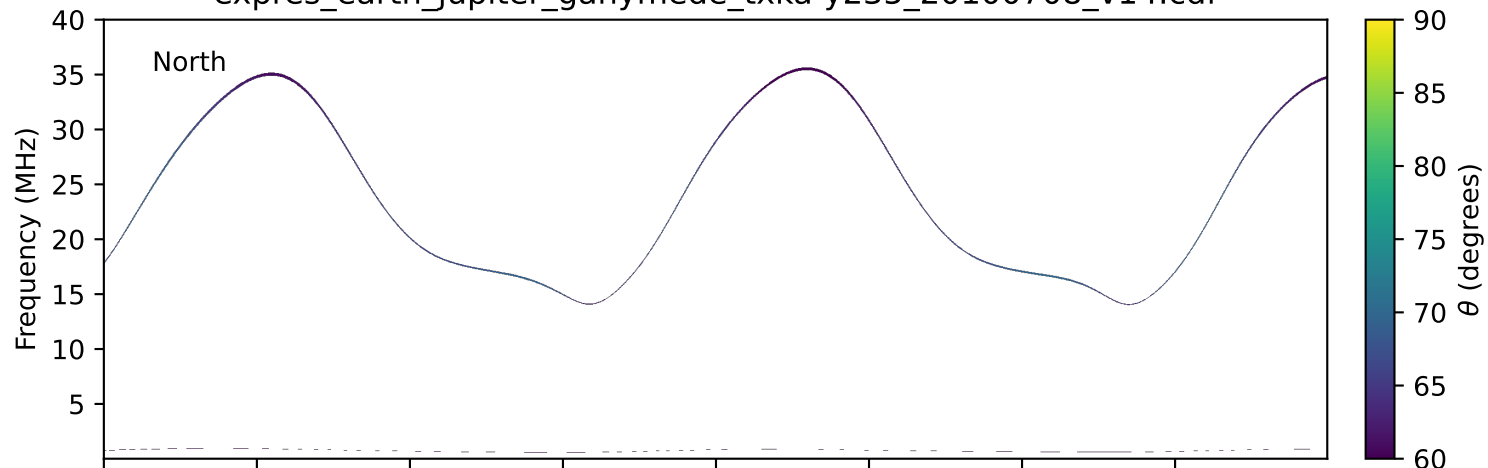
expres_earth_jupiter_ganymede_txka-y235_20100708_v14.cdf
