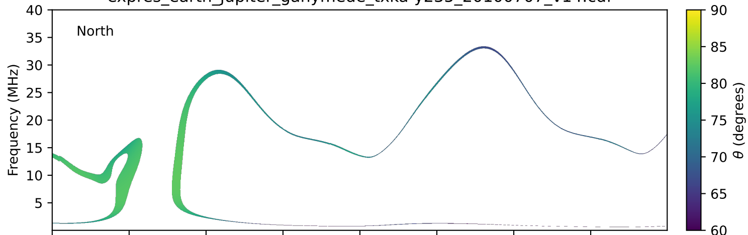
expres_earth_jupiter_ganymede_txka-y235_20100707_v14.cdf
