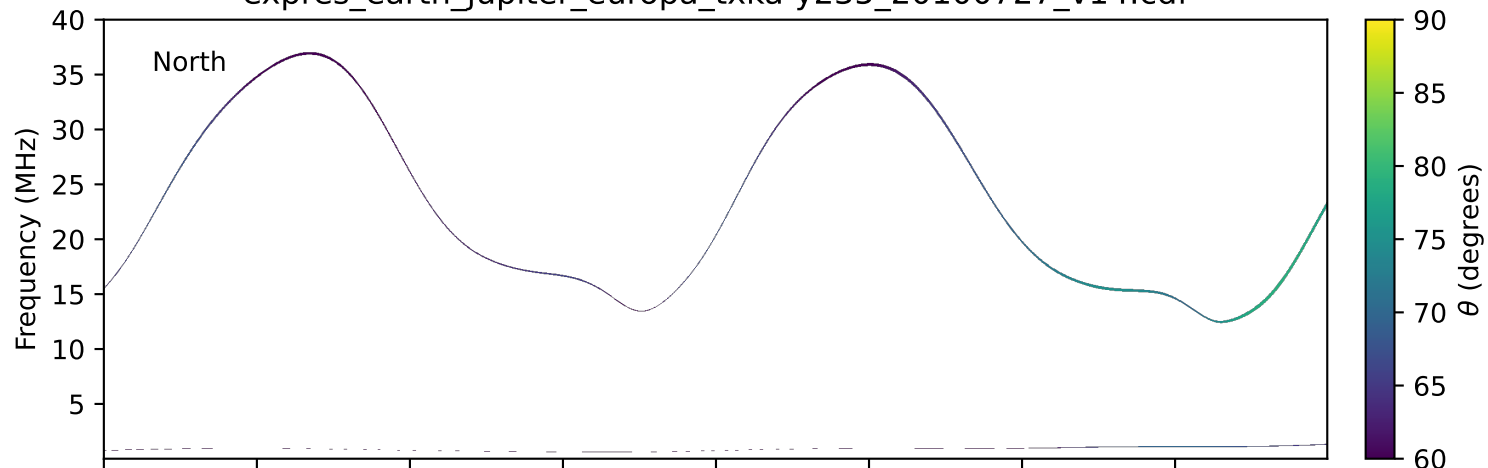
expres_earth_jupiter_europa_txka-y235_20100727_v14.cdf
