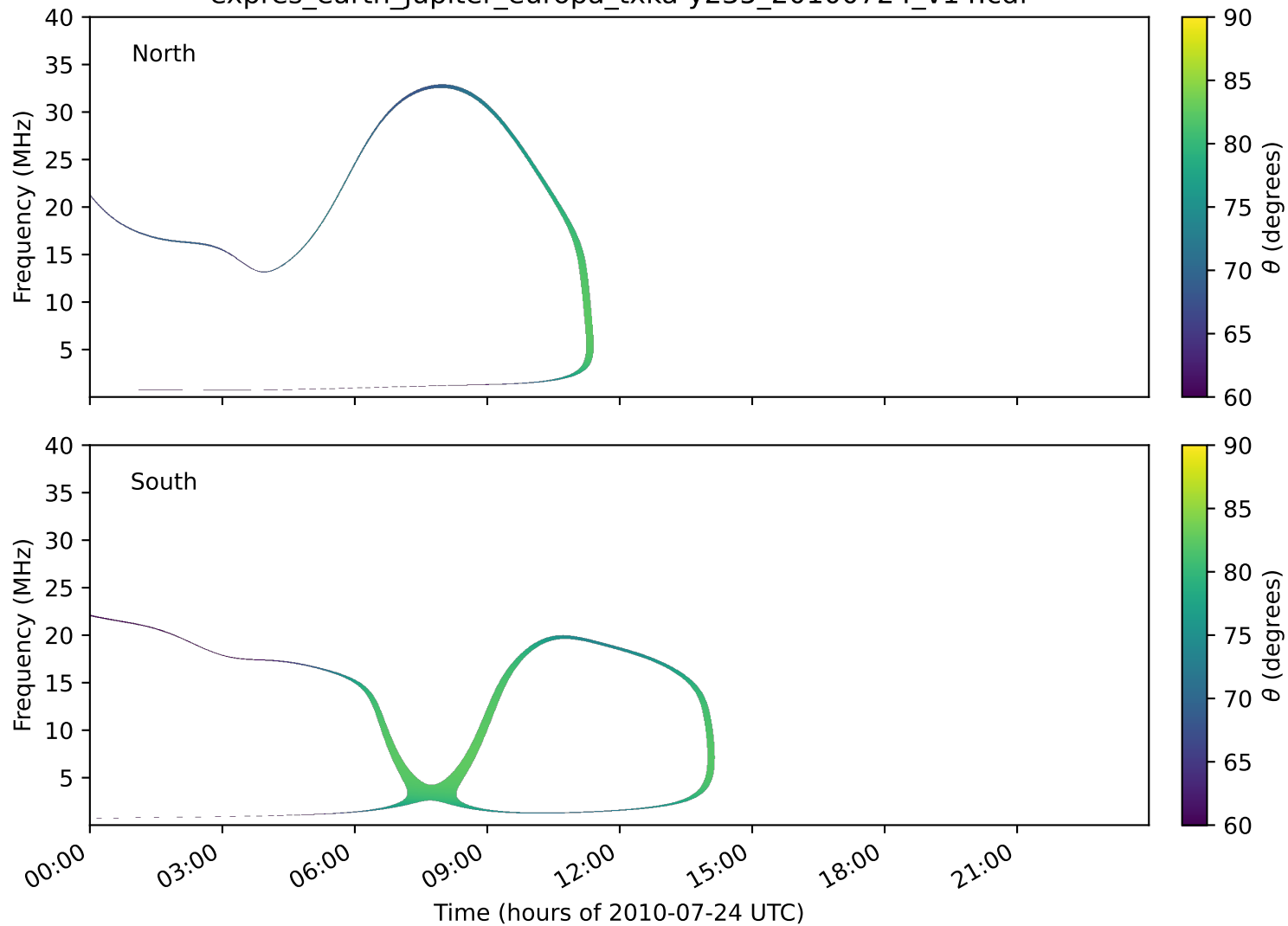
expres_earth_jupiter_europa_txka-y235_20100724_v14.cdf
