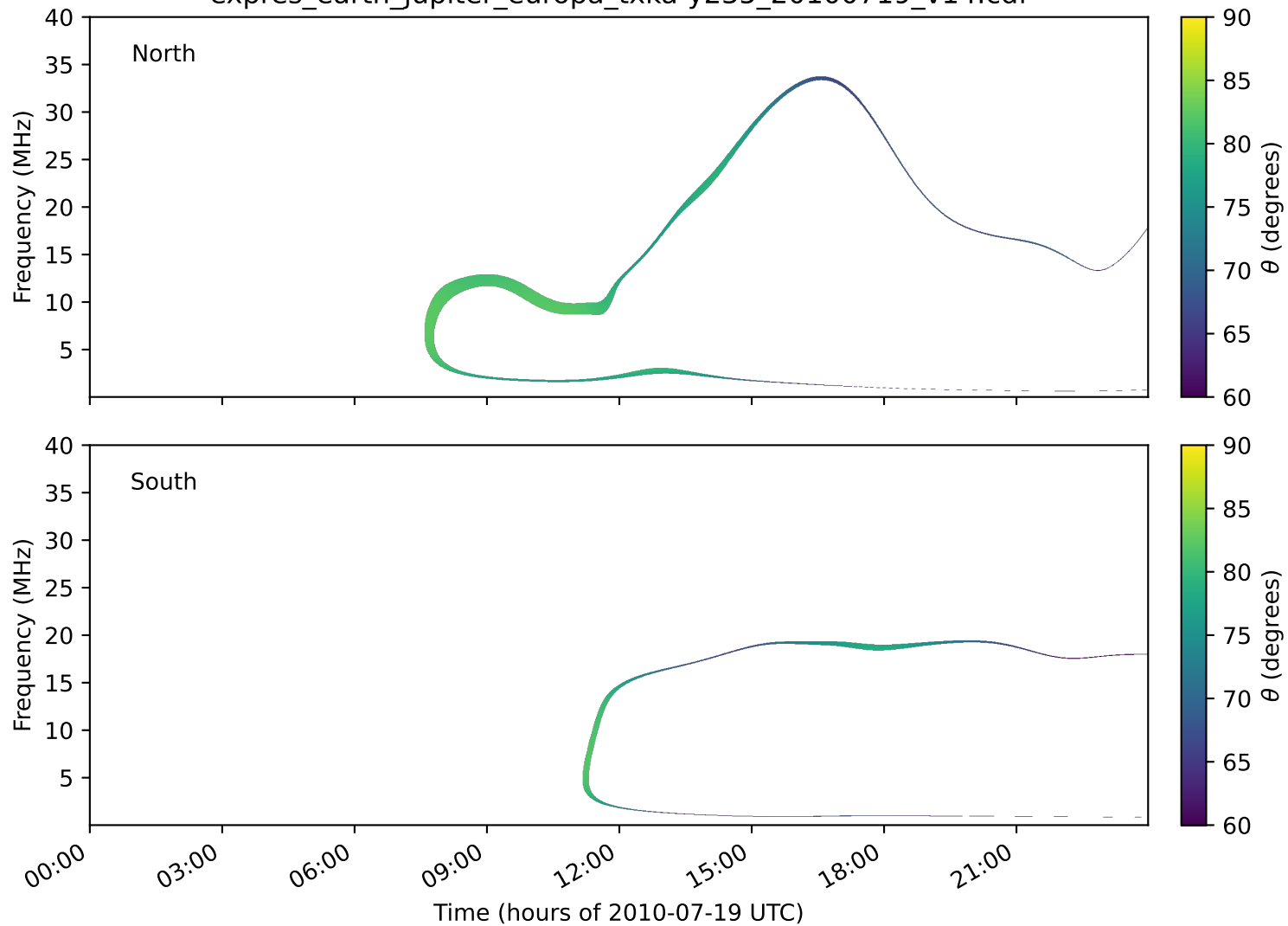
expres_earth_jupiter_europa_txka-y235_20100719_v14.cdf
