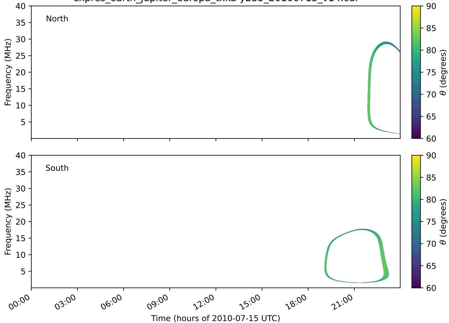
expres_earth_jupiter_europa_txka-y235_20100715_v14.cdf
