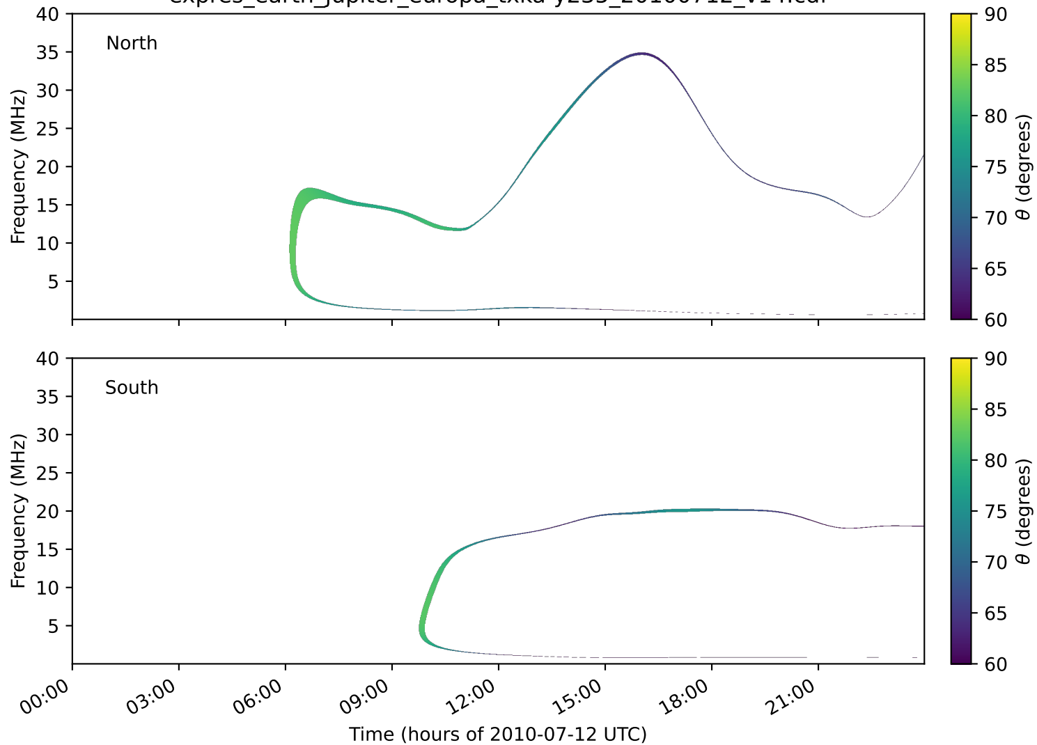
expres_earth_jupiter_europa_txka-y235_20100712_v14.cdf
