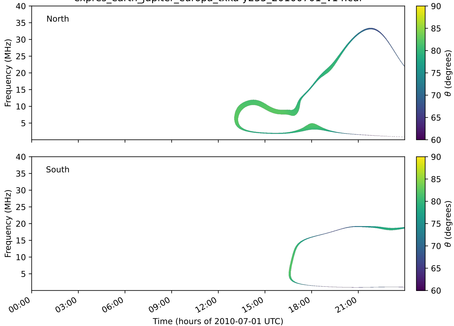
expres_earth_jupiter_europa_txka-y235_20100701_v14.cdf
