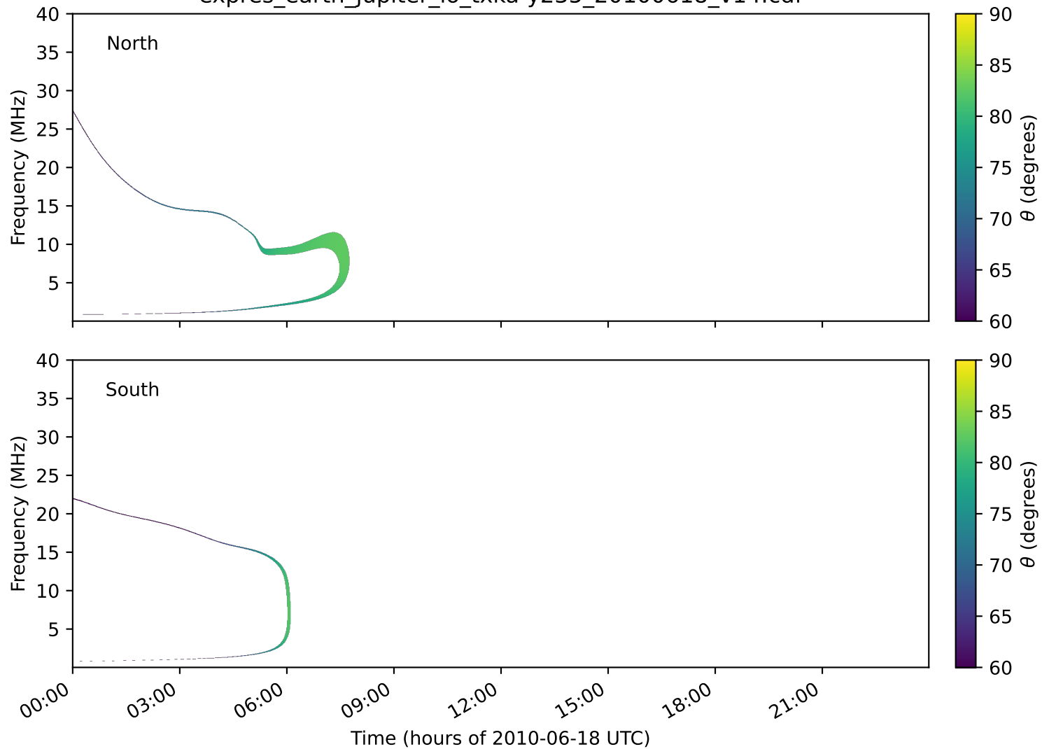
expres_earth_jupiter_io_txka-y235_20100618_v14.cdf
