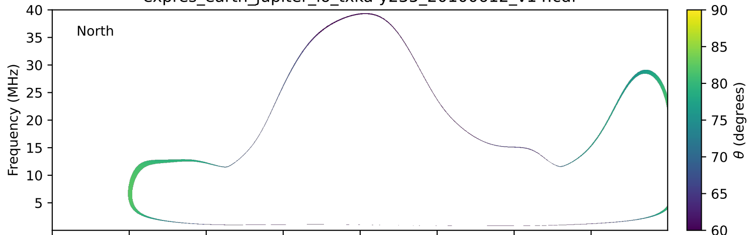
expres_earth_jupiter_io_txka-y235_20100612_v14.cdf
