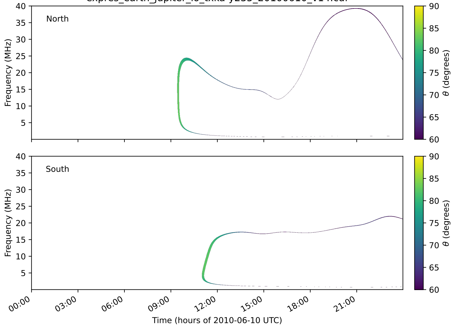
expres_earth_jupiter_io_txka-y235_20100610_v14.cdf
