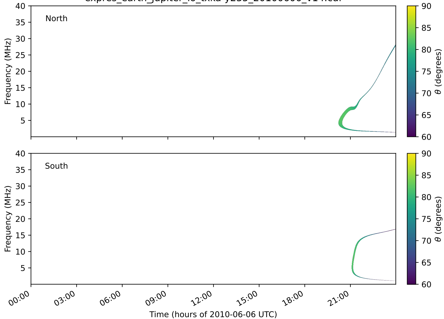
expres_earth_jupiter_io_txka-y235_20100606_v14.cdf
