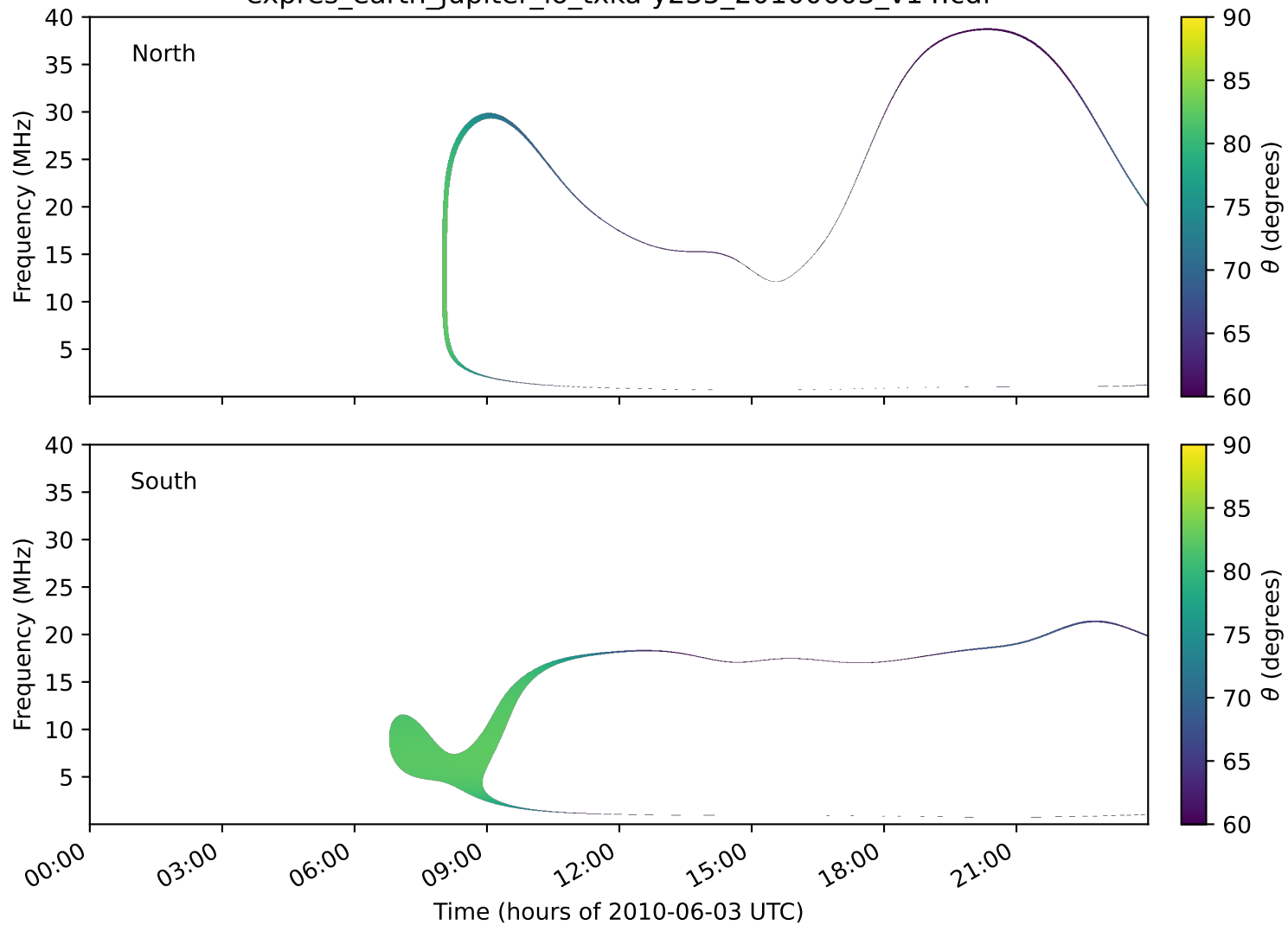
expres_earth_jupiter_io_txka-y235_20100603_v14.cdf
