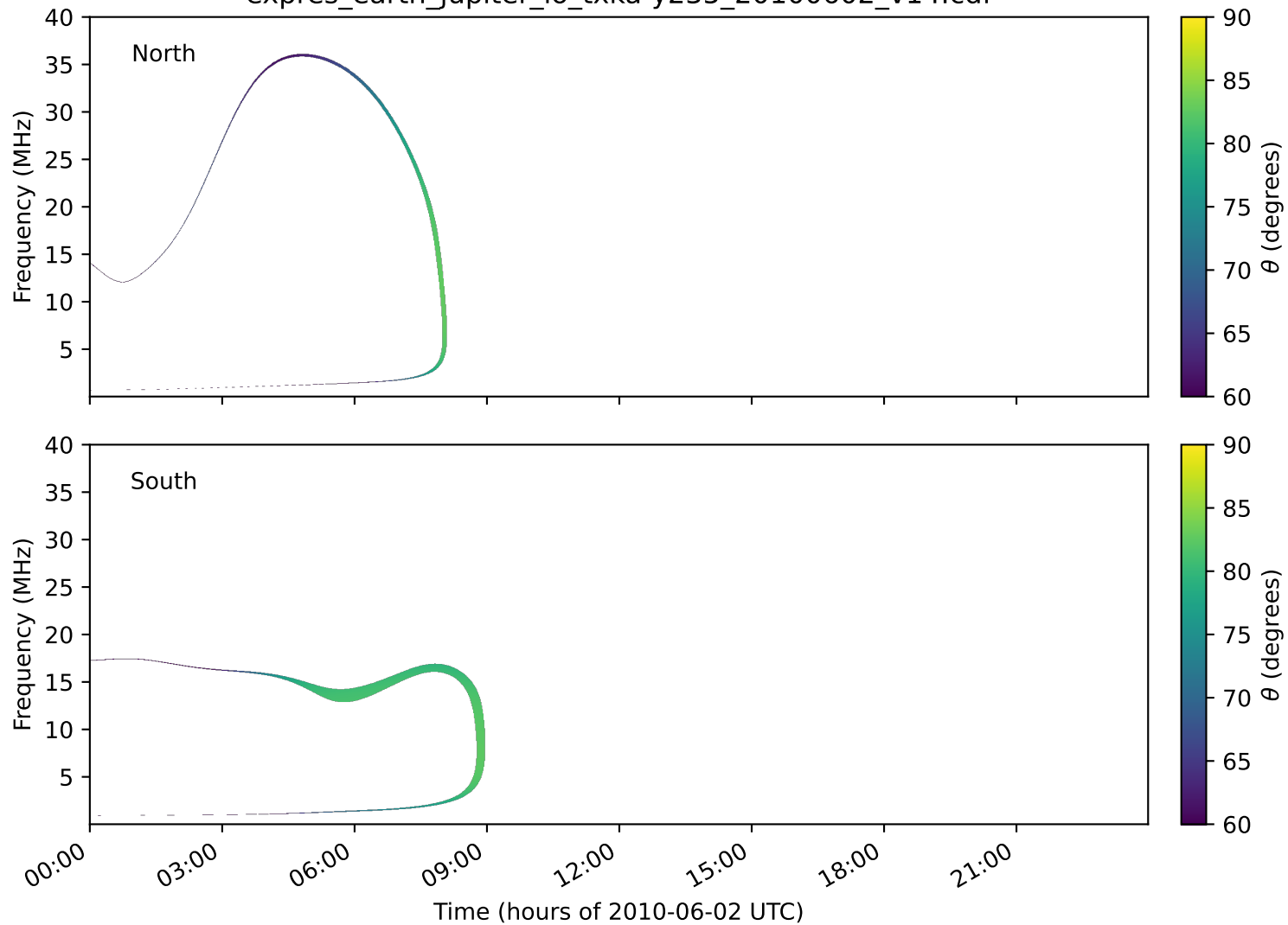
expres_earth_jupiter_io_txka-y235_20100602_v14.cdf
