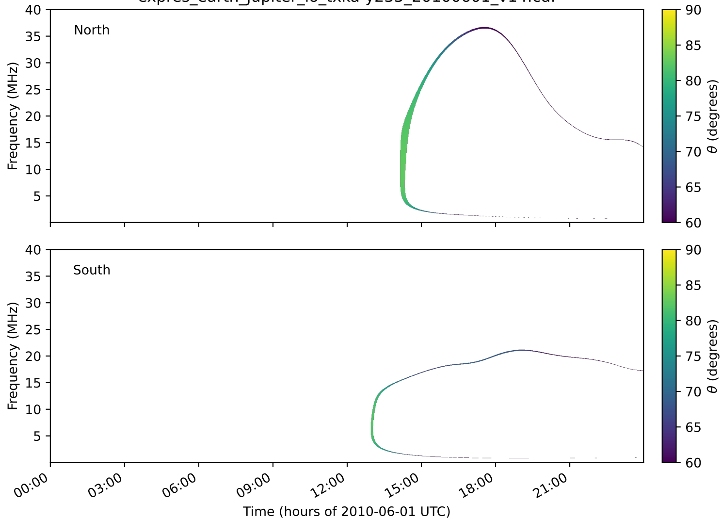
expres_earth_jupiter_io_txka-y235_20100601_v14.cdf
