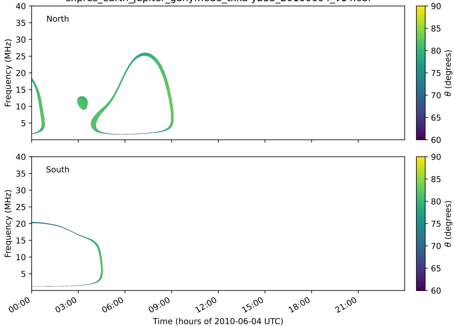
expres_earth_jupiter_ganymede_txka-y235_20100604_v14.cdf
