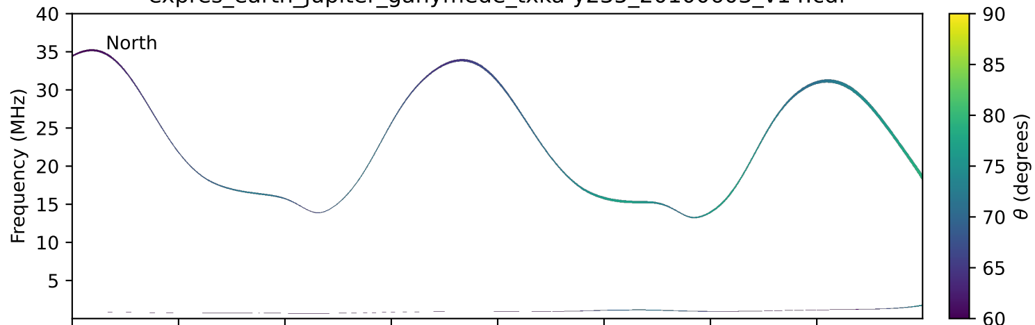
expres_earth_jupiter_ganymede_txka-y235_20100603_v14.cdf
