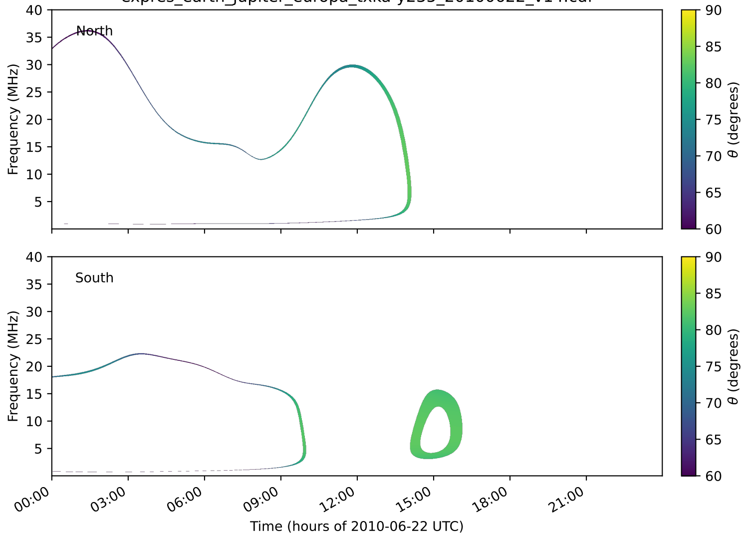
expres_earth_jupiter_europa_txka-y235_20100622_v14.cdf
