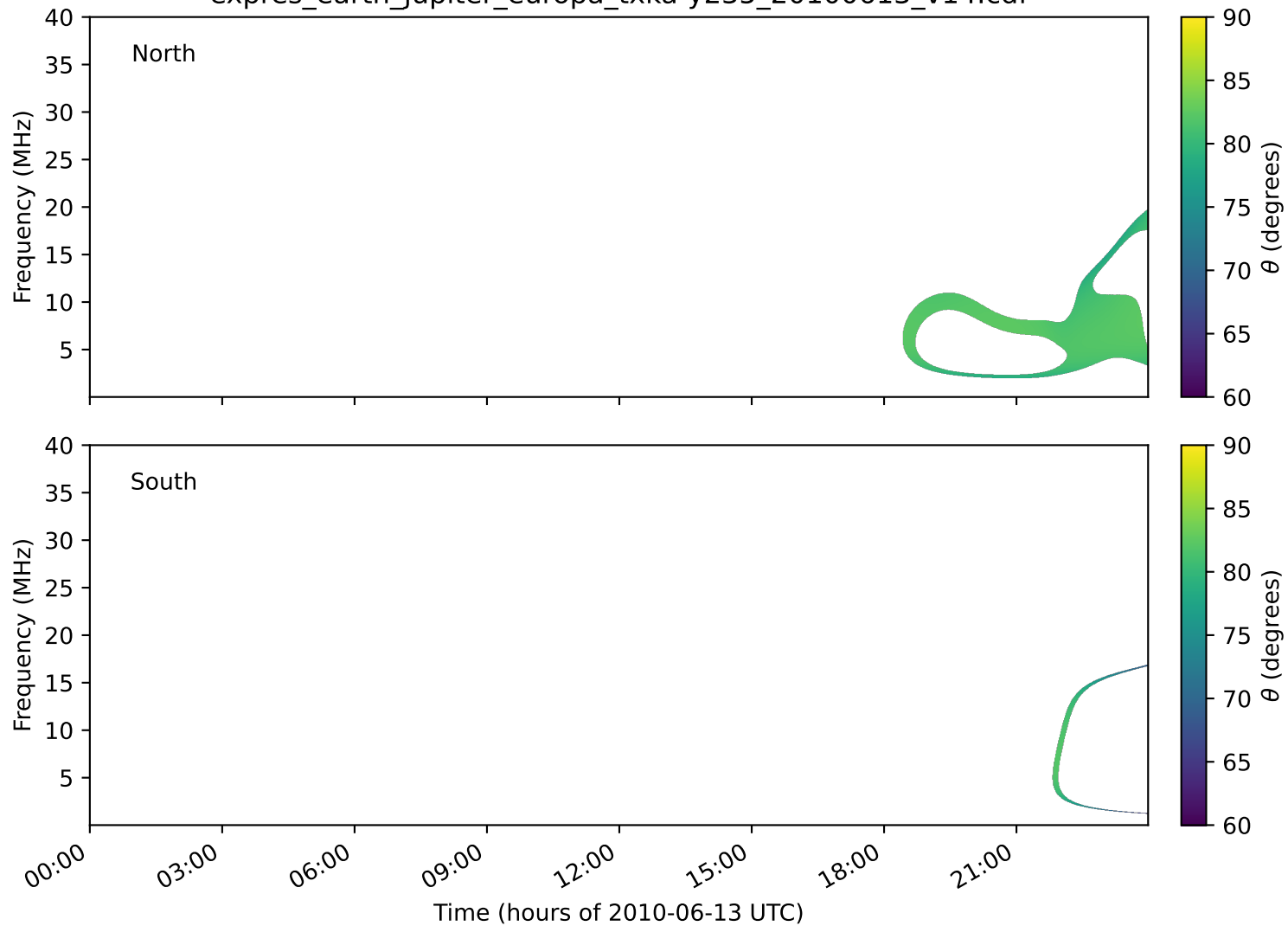
expres_earth_jupiter_europa_txka-y235_20100613_v14.cdf
