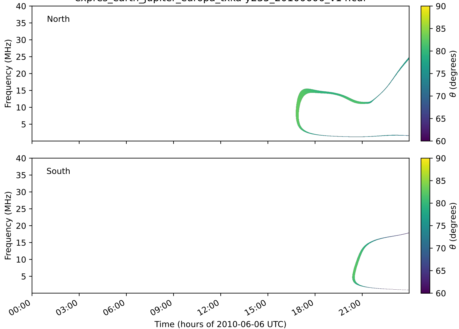
expres_earth_jupiter_europa_txka-y235_20100606_v14.cdf
