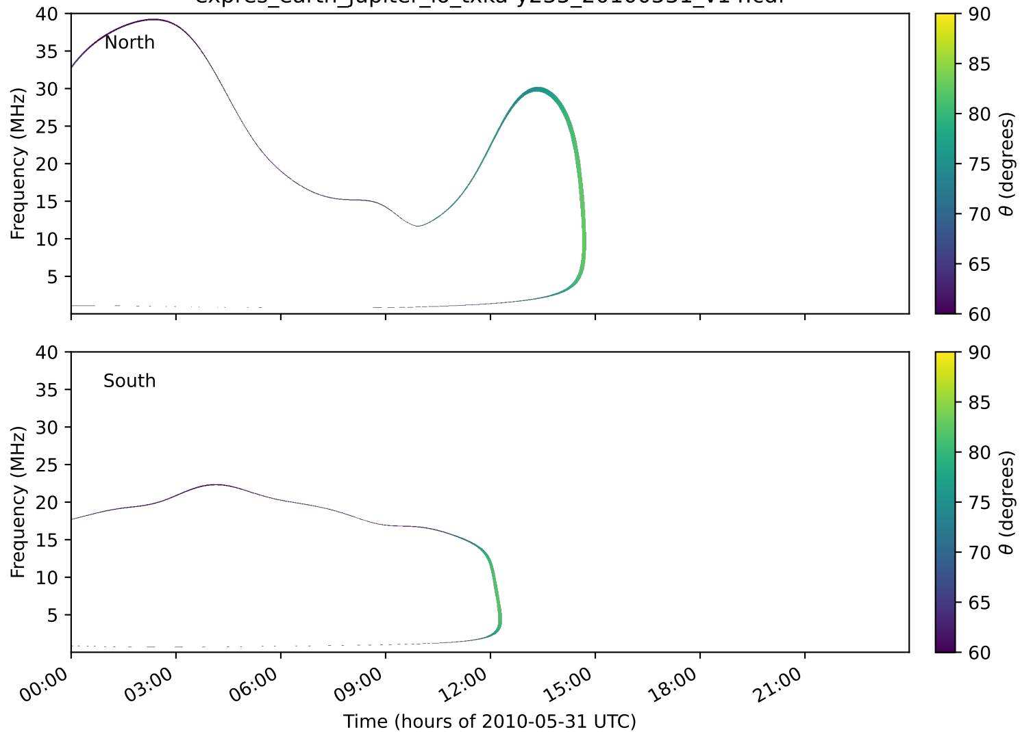
expres_earth_jupiter_io_txka-y235_20100531_v14.cdf
