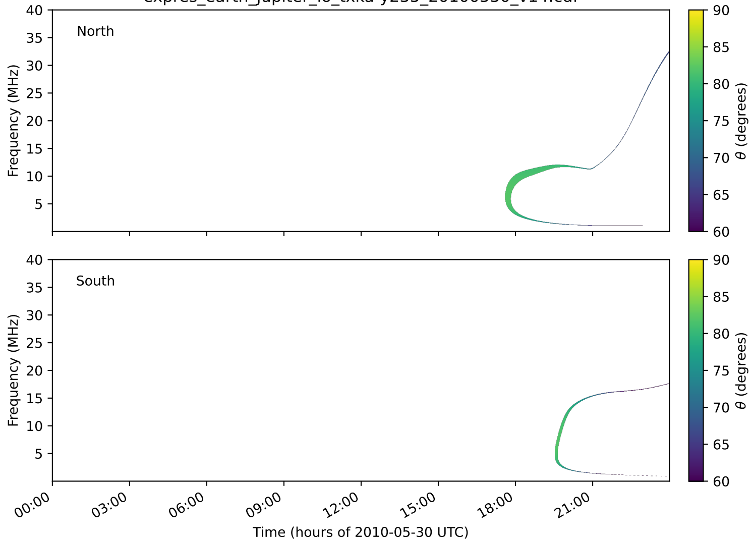
expres_earth_jupiter_io_txka-y235_20100530_v14.cdf
