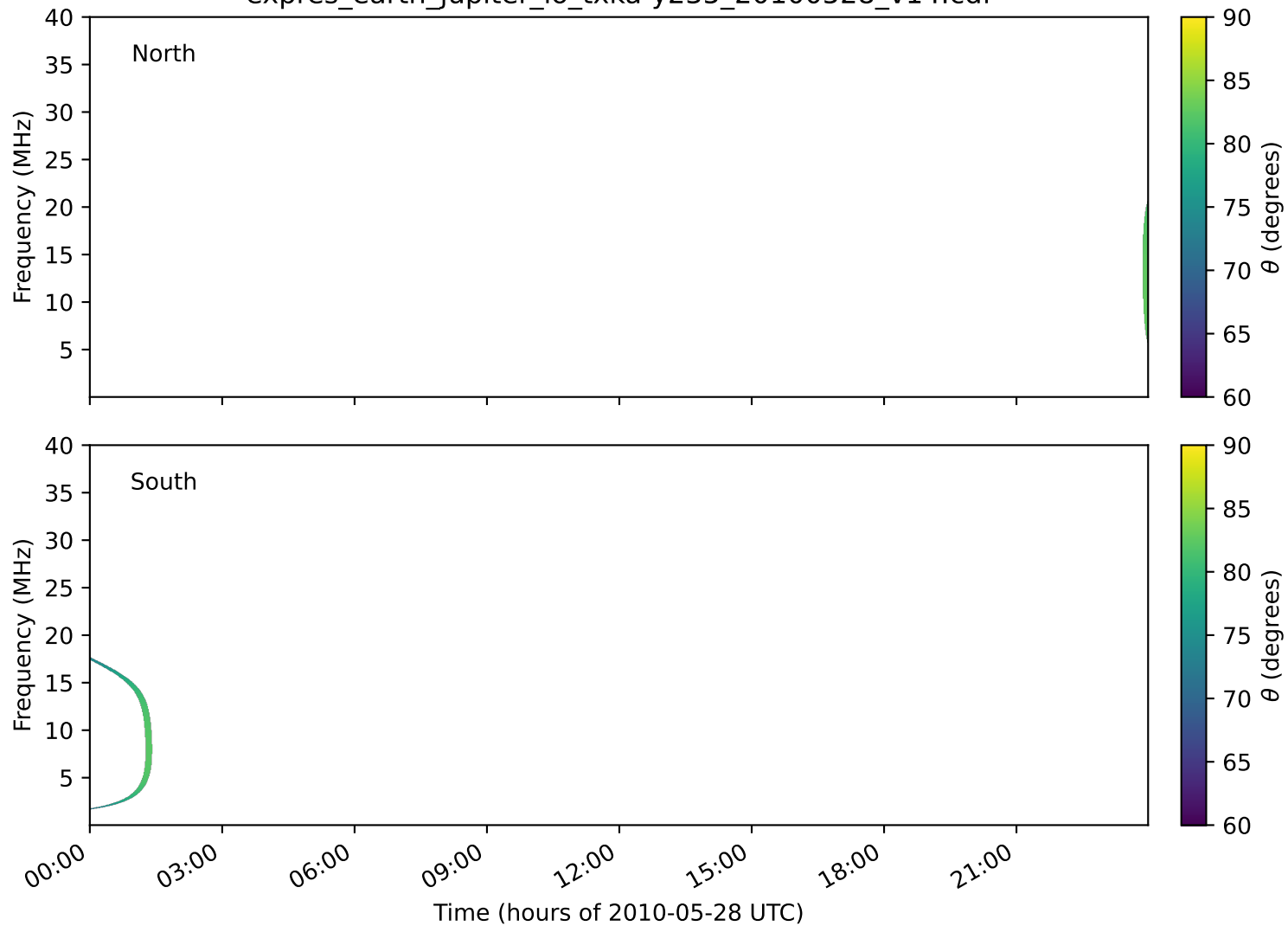
expres_earth_jupiter_io_txka-y235_20100528_v14.cdf
