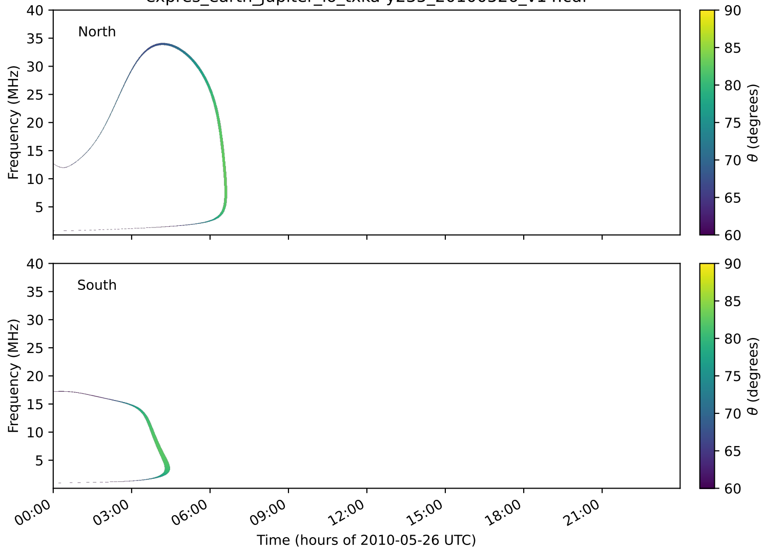
expres_earth_jupiter_io_txka-y235_20100526_v14.cdf
