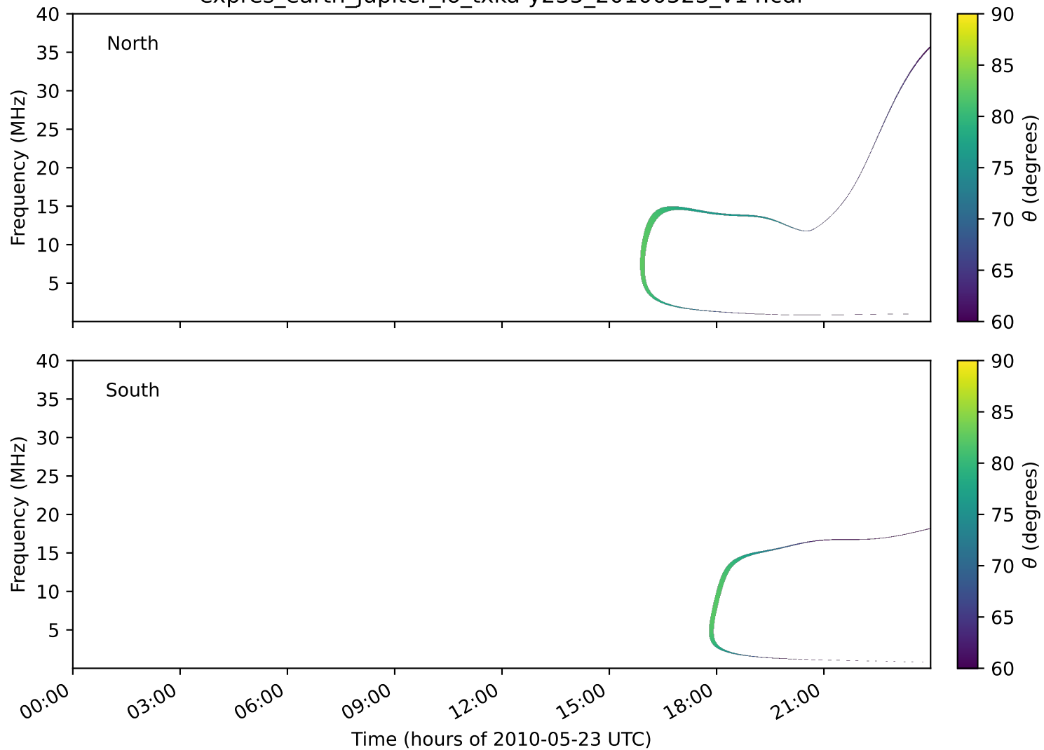
expres_earth_jupiter_io_txka-y235_20100523_v14.cdf
