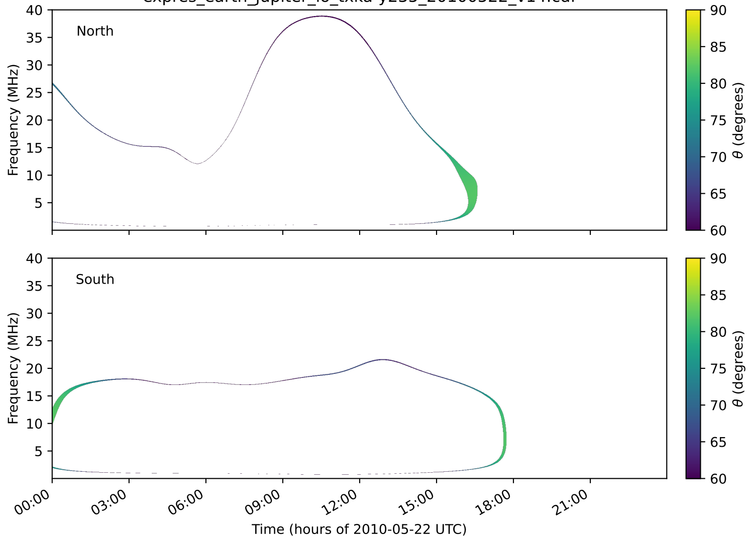
expres_earth_jupiter_io_txka-y235_20100522_v14.cdf
