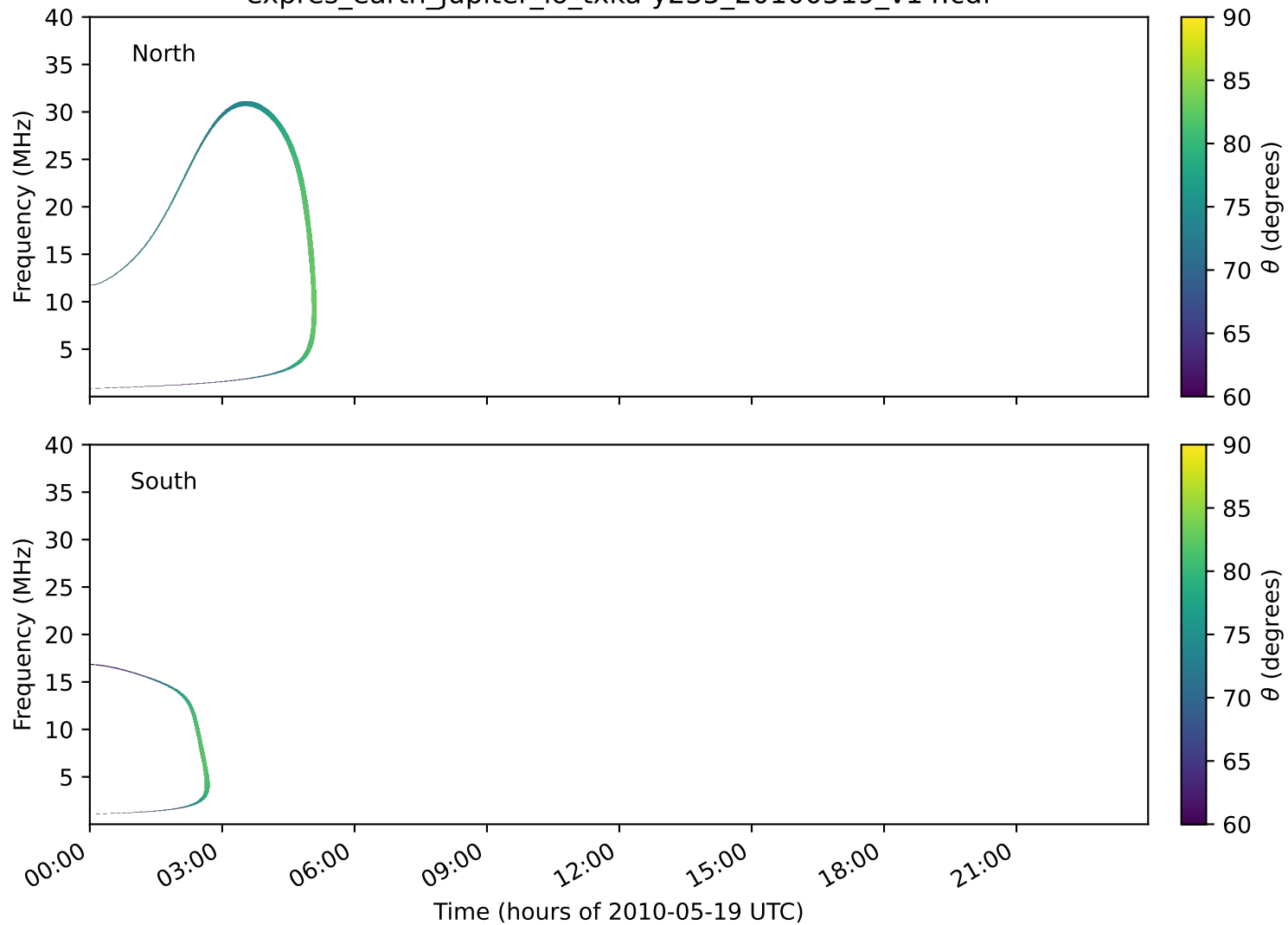
expres_earth_jupiter_io_txka-y235_20100519_v14.cdf
