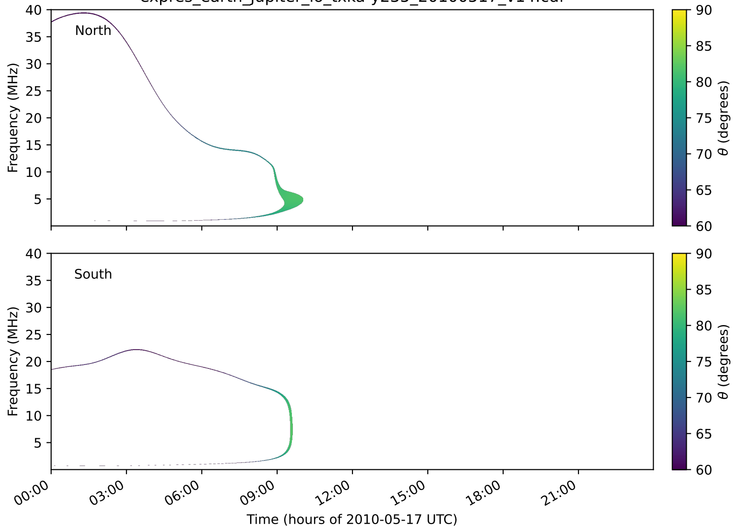
expres_earth_jupiter_io_txka-y235_20100517_v14.cdf
