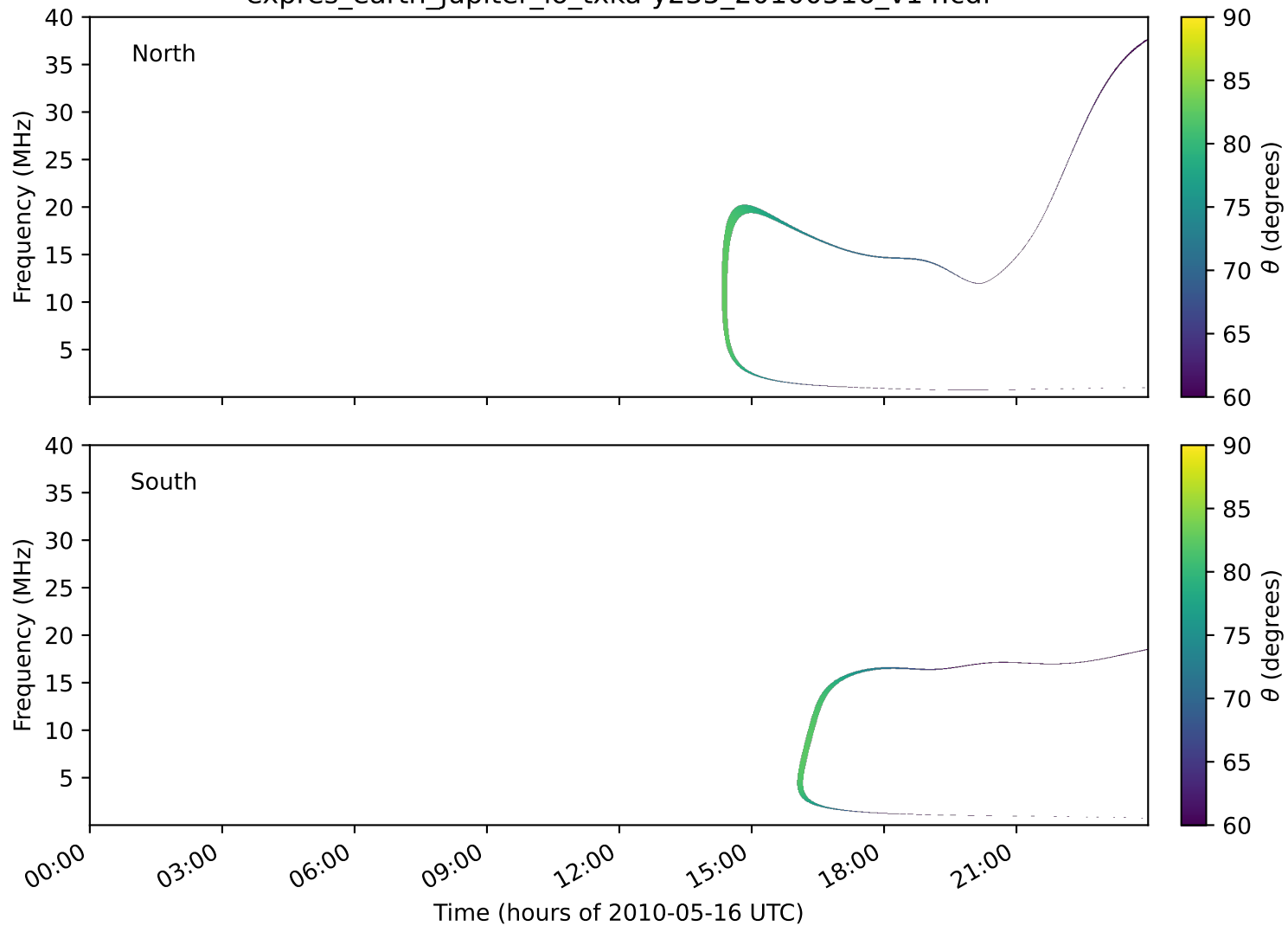
expres_earth_jupiter_io_txka-y235_20100516_v14.cdf
