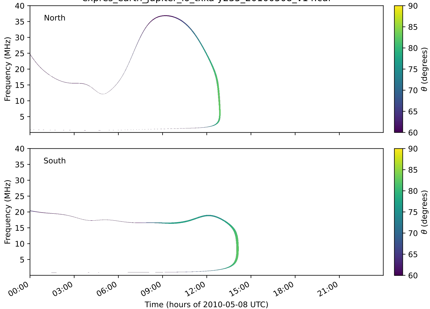
expres_earth_jupiter_io_txka-y235_20100508_v14.cdf
