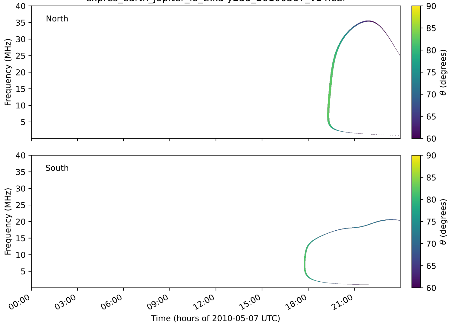
expres_earth_jupiter_io_txka-y235_20100507_v14.cdf
