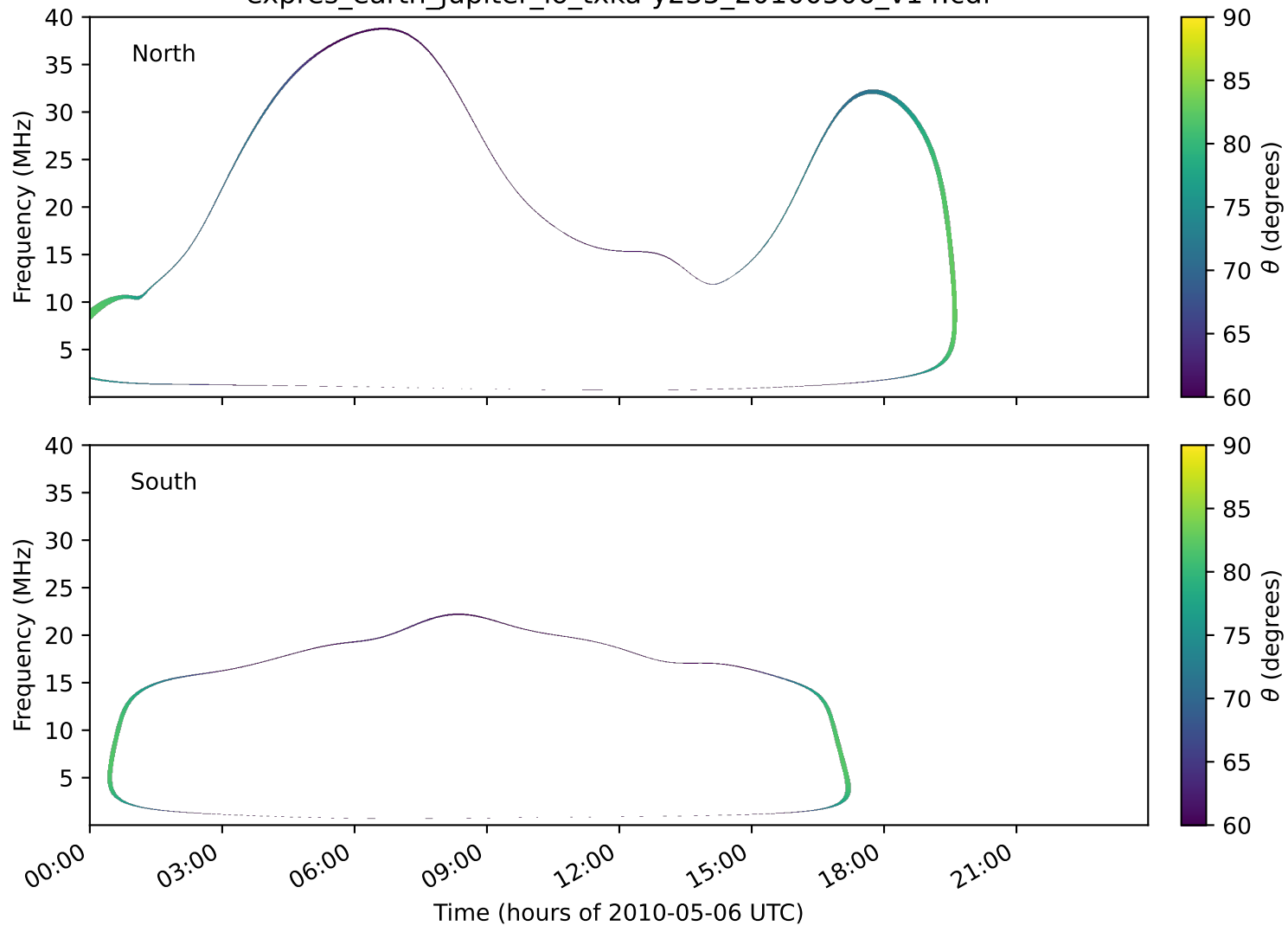
expres_earth_jupiter_io_txka-y235_20100506_v14.cdf
